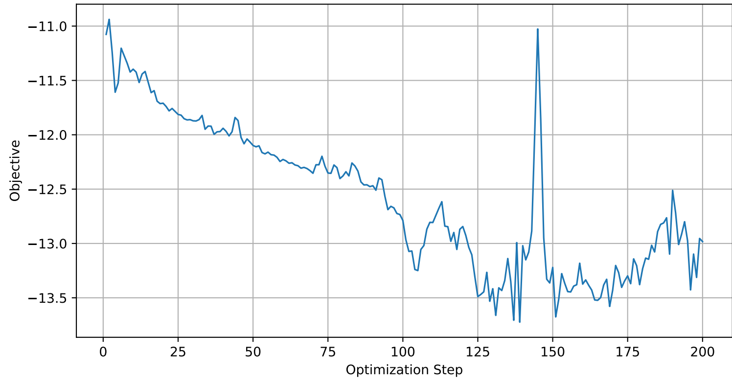
Loss History
